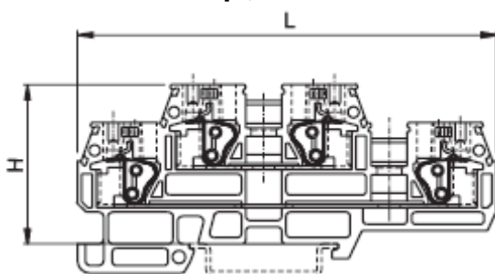
Nq2,5-3-G Nq2,5-3-BL
