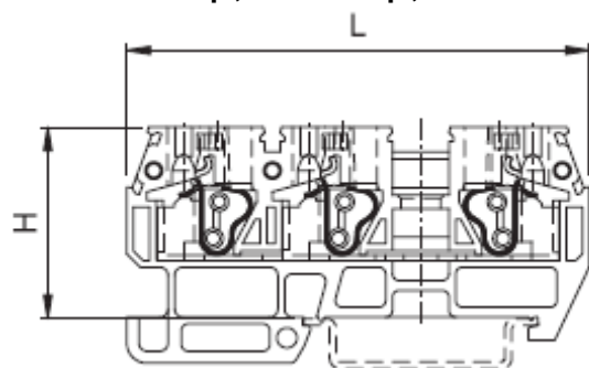
Euro QM 1/2-2,5/35 Nq2,5-1-G & Nq2,5-1-BL
